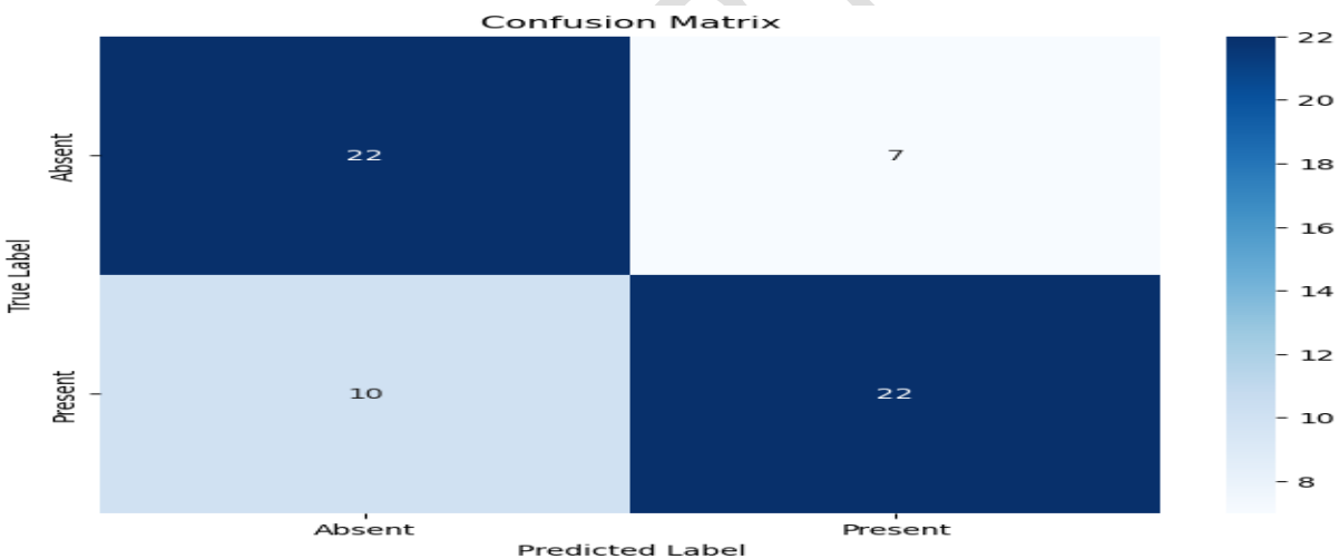
Figure 10: Confusion matrix for the performances using Decision Tree procedure.
