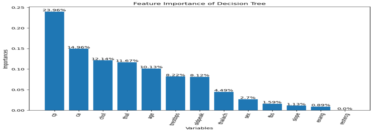
Figure 11: Features Importance
