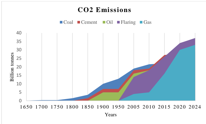
Fig. 1. Carbon dioxide emissions by fuel type, globally
