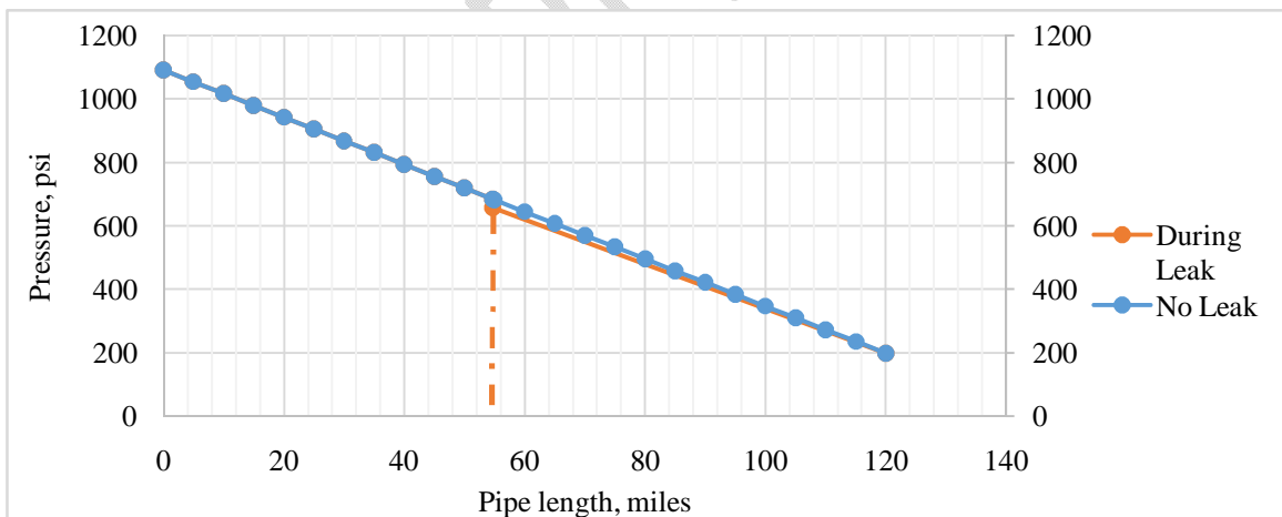
Figure 9: Pressure profile for case 4 during leak and in the absence of leak
