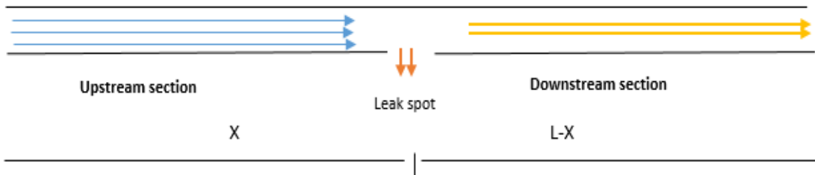
Figure 3: Pipeline Schematics for Determination in the presence of Leak
