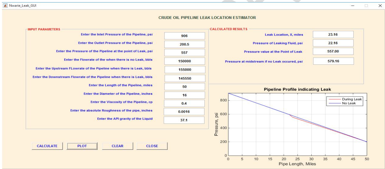
Figure 5: Crude oil pipeline Leak location Estimator (Matlab GUI)
