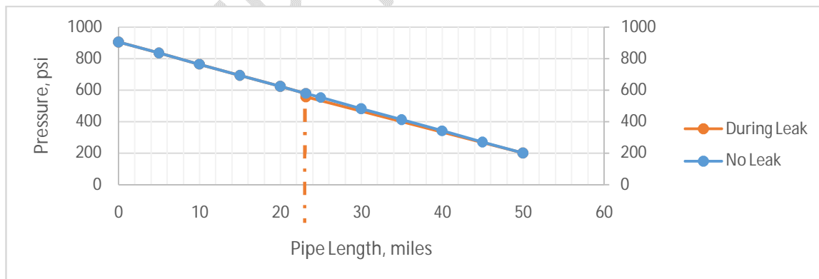
Figure 6: Pressure profile for case 1 during leak and in the absence of leak
