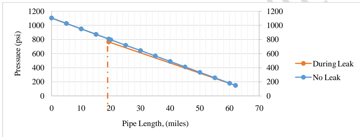
Figure 7: Pressure profile for case 2 during leak and in the absence of leak
