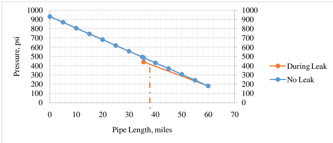
Figure 8: Pressure profile for case 3 during leak and in the absence of leak
