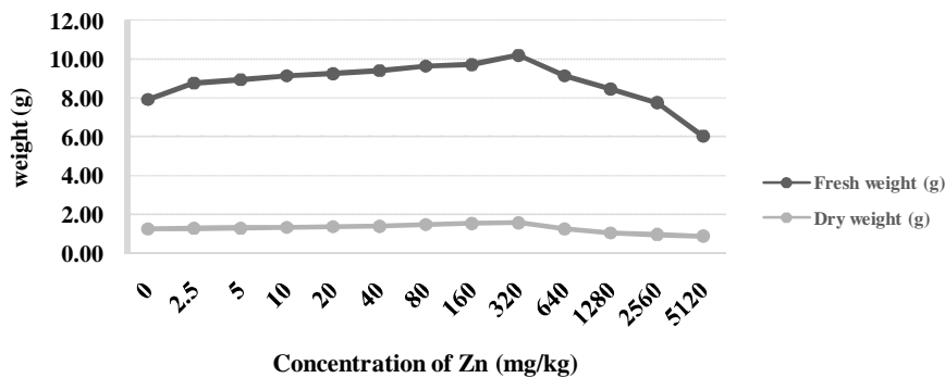
Figure 5: Effect of different concentration of seed priming of ZnO NPs on seedling fresh and dry weight of maize seedlings after priming
