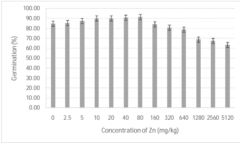
Figure 3: Effect of different concentration of seed priming of ZnO NPs on germination maize seeds after priming
