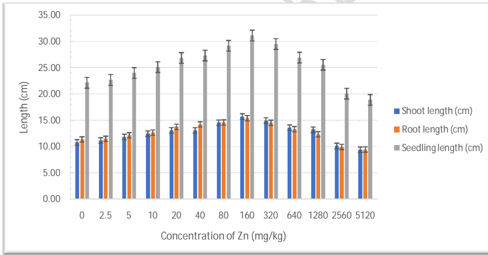
Figure 4: Effect of different concentration of seed priming of ZnO NPs on Shoot, root and seedling length of maize after priming
