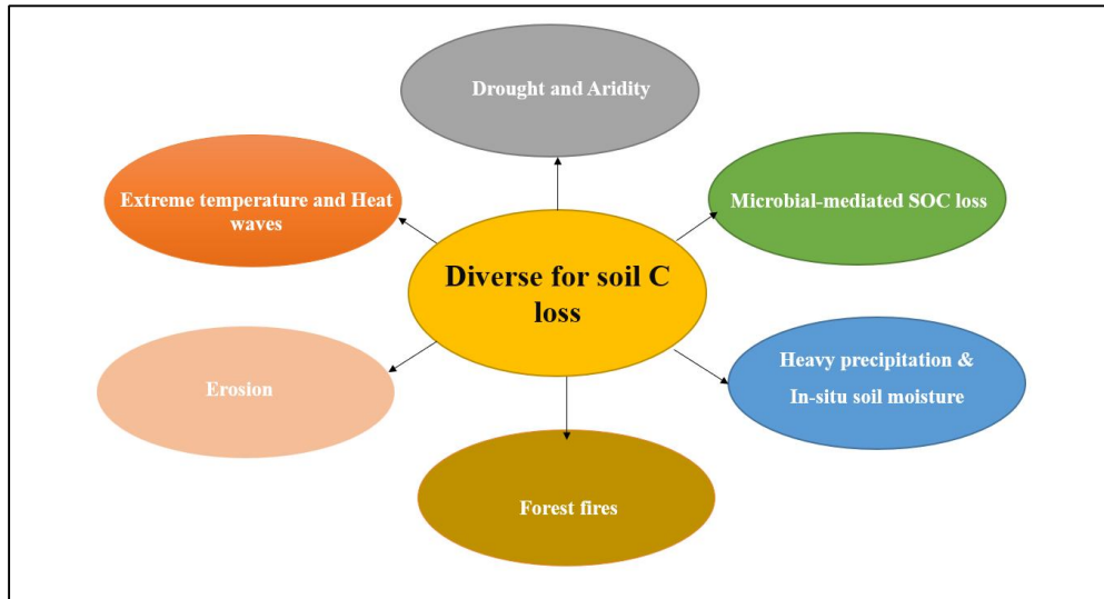
Fig 1: Different divers for climate-induced Soil carbon loss
