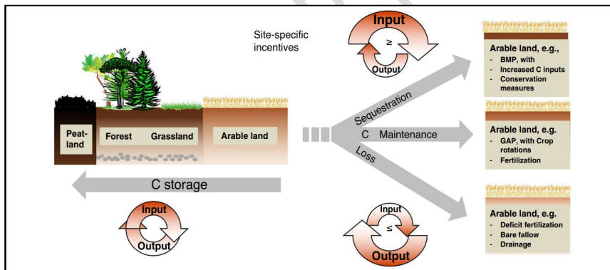
Fig2: The loss of C after conversion of native ecosystems i.e. peat land, forest, and grassland to arable land {adopted from Amelunget et al. , (2020) 11:5427 | https://doi.org/10.1038/s41467-020-18887-7 }
