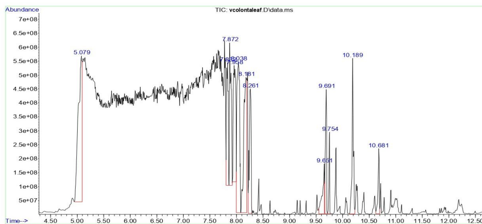
Figure 4: Chromatogram of the dichloromethane leaf extract of V. colorata
