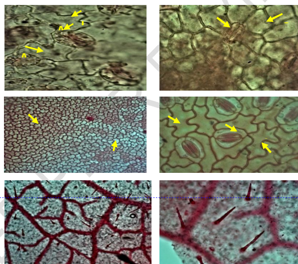
Figure 1. (A): C. colorata Adaxial surface ×10 (IEC: Irregular Epidermal Cell; AnoS; Anomocytic stomata; AbS; Abnormal stomata; (B): C. colorata Abaxial surface ×10 (IEC: Irregular Epidermal Cell; AnoS; Anomocytic stomata. (C) C. conferta Adaxial surface ×4 (UAWP: Undulate anticlinal wall pattern; IEC; Irregular Epidermal Cell. (D) C. conferta Abaxial surface ×10 (SAWP: Sinuous Anticlinal Wall Pattern; PS; Parasitic stomata; IEC: Irregular Epidermal Cell. (E) C. conferta (UT: Unicellular trichome; Bfk: Biforked termination, QAe; Quadrangular aereolation, LT; Linear vein termination. (F) C. conferta Abaxial surface ×10 (UT; Unicellular trichome
