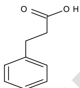
Hydrocinnamic acid
