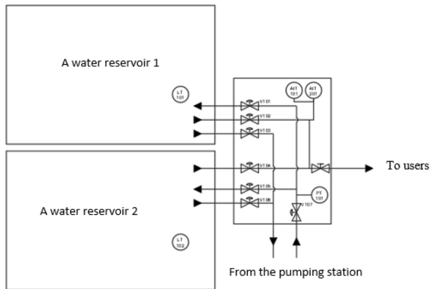
Figure 2. The scheme of entering and distributing water from the pumping station to the reservoirs
