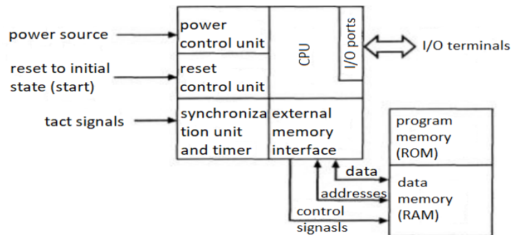
Figure 1. Block diagram of a microcontroller with external memory
