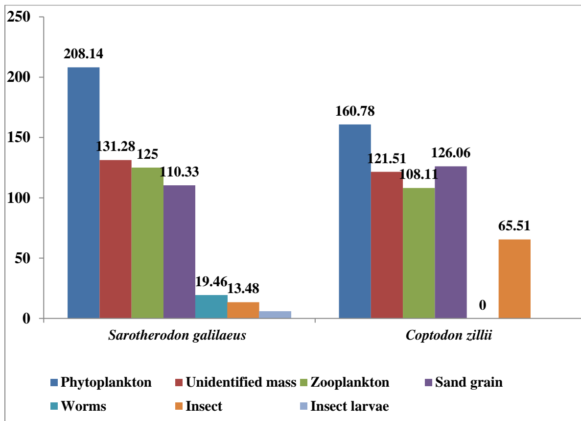
Figure2: The index of relative importance (IRI) of the food items in the diet of 2 dominant fish species from Ado-Ekiti Reservoir
