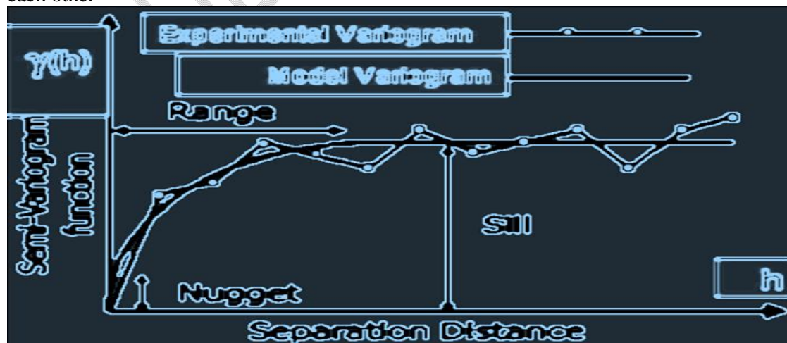
Fig 4: Parameters of Semi-Variogram
