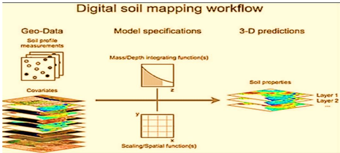
Fig 5. Workflow of digital soil mapping
