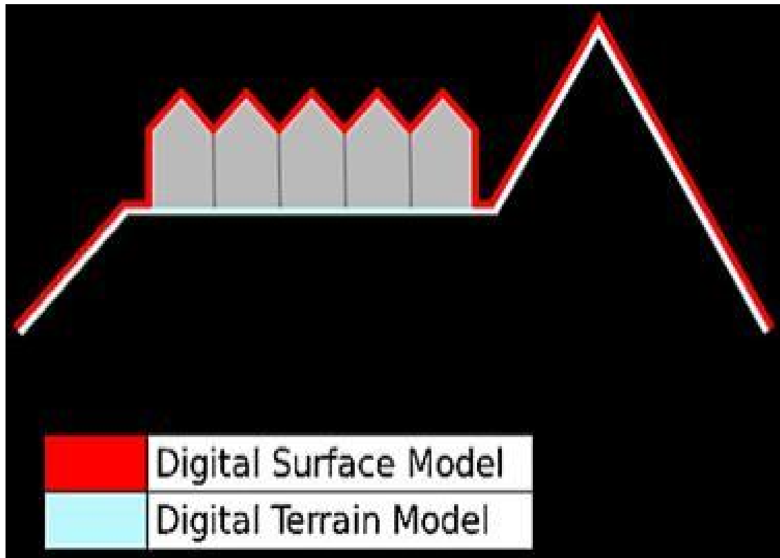
Fig 2: Pictorial representation of digital elevation model
