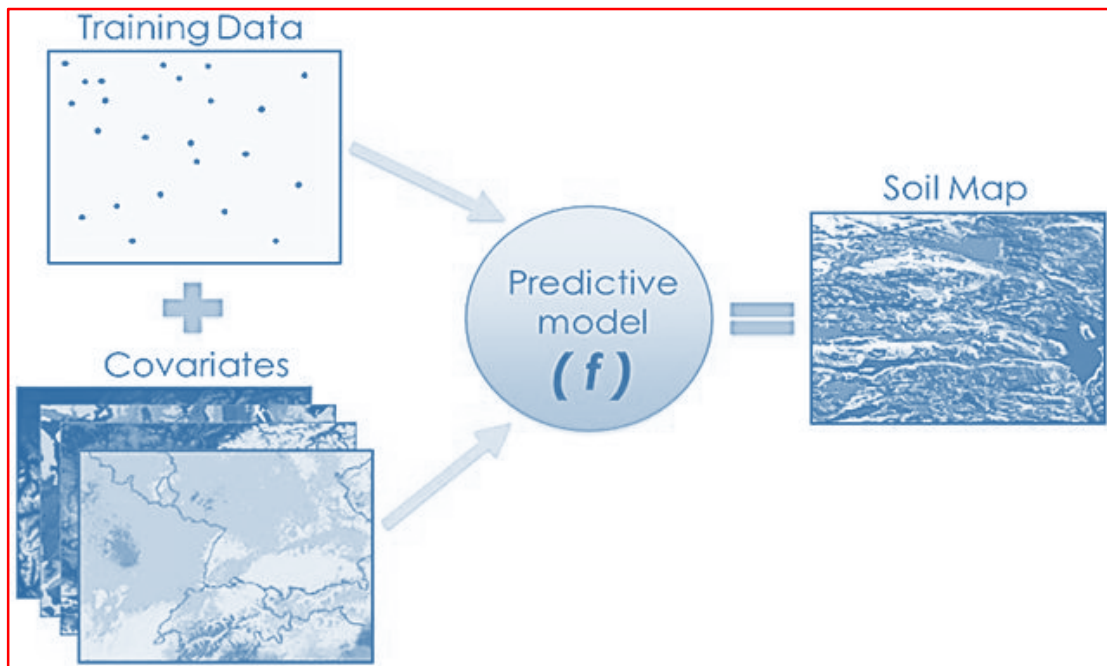
Fig 1: Pictorial representation of digital soil mapping
