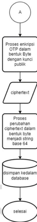
Figure 8. Encryption Flowchart
