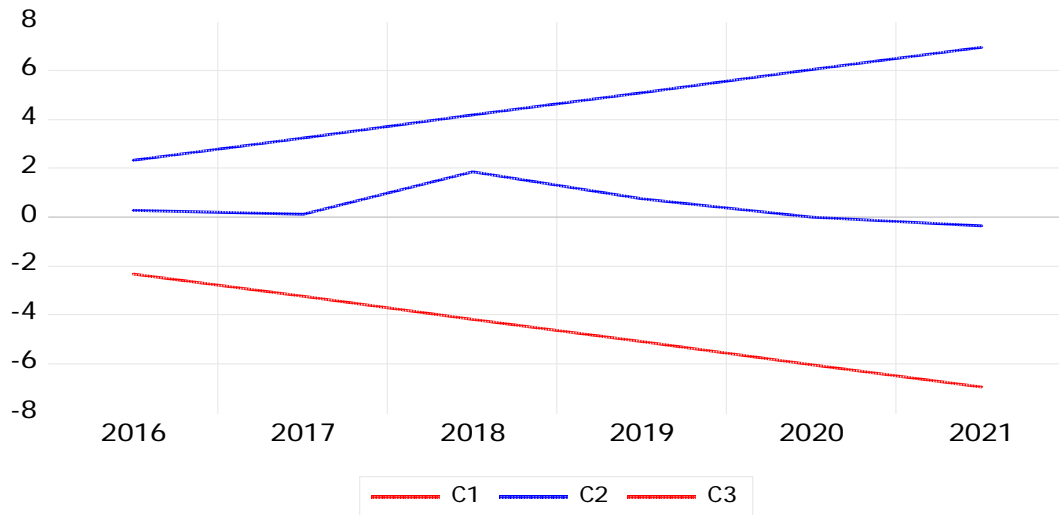
Figure 1: CUSUM Test for Model Stability
