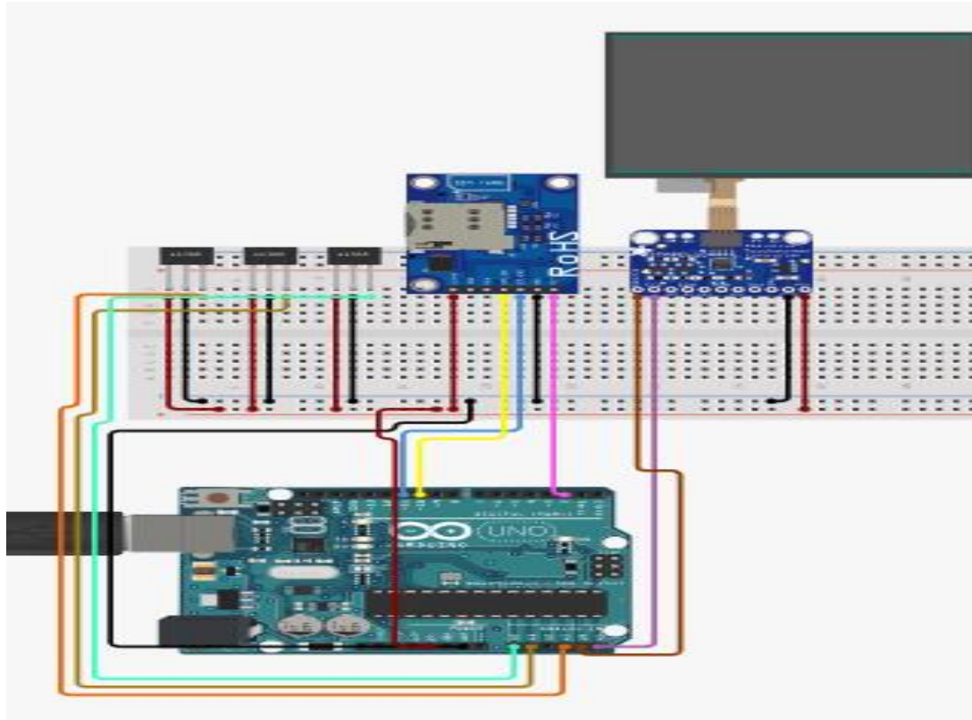
Figure 2 Complete Magnetic field sensor design for Pipeline Monitoring System.
