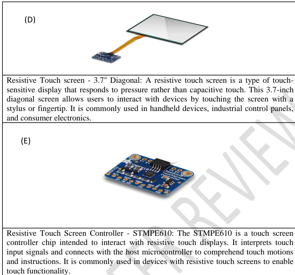
Figure 1 The various components used for the detection of leak, corrosion of the Petroleum Monitoring System
