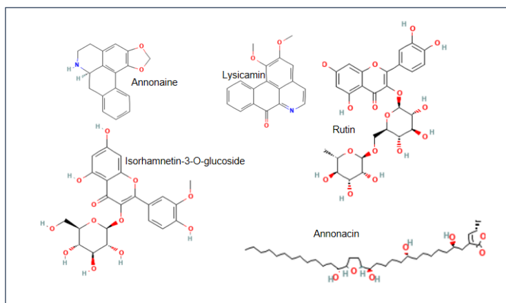
Figure 3: Some prevalent phytoconstituents found in A. stenophylla
