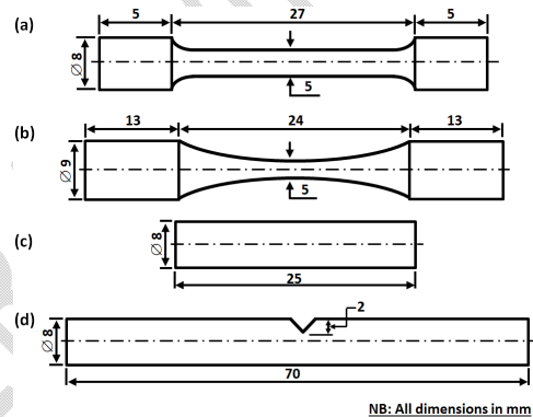
Figure 1: Schematic diagrams of the machined (a) tensile; (b) fatigue; (c) compression and (d) impact tests specimens
