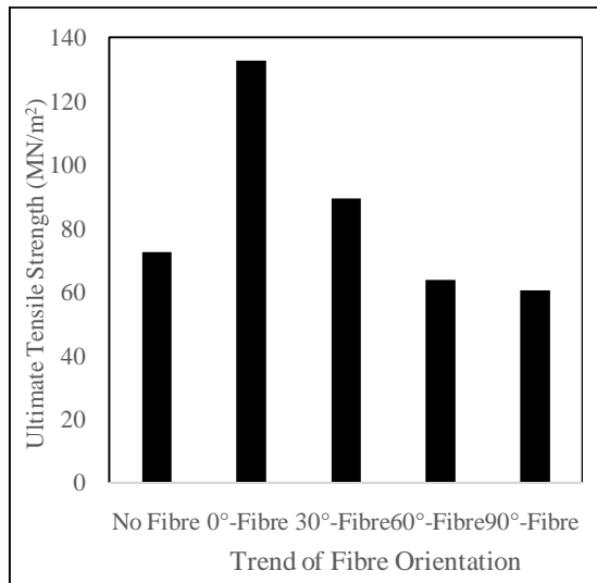
Figure 4: Plot of ultimate tensile strength versus trend of fibre orientation
