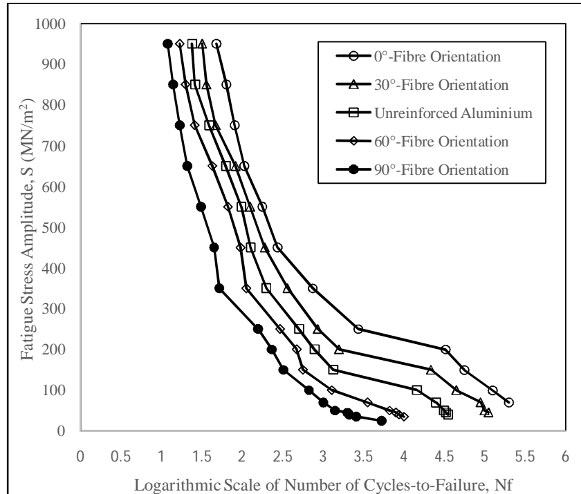
Figure 6: Plot of fatigue stress amplitude versus logarithmic scale of number of cycles-to-failure for the specimens
