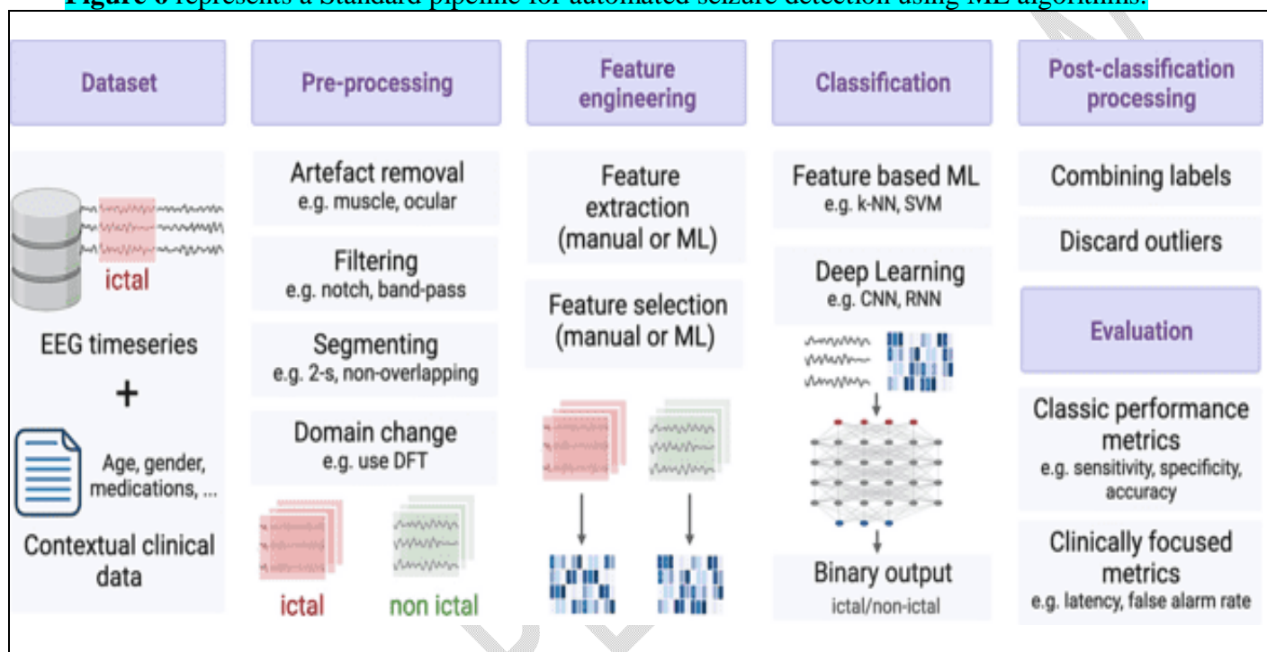
Figure 6. Standard pipeline for automated seizure detection using ML algorithms [6]
