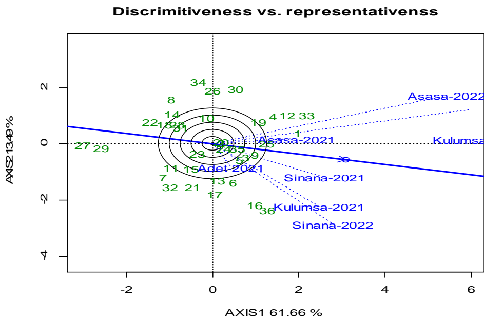
Figure 3. GGE-biplot for comparing the environments with the ideal environment
