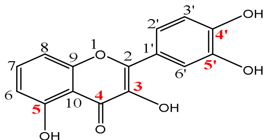
Fig. 11 : Flavonoids basic structure
