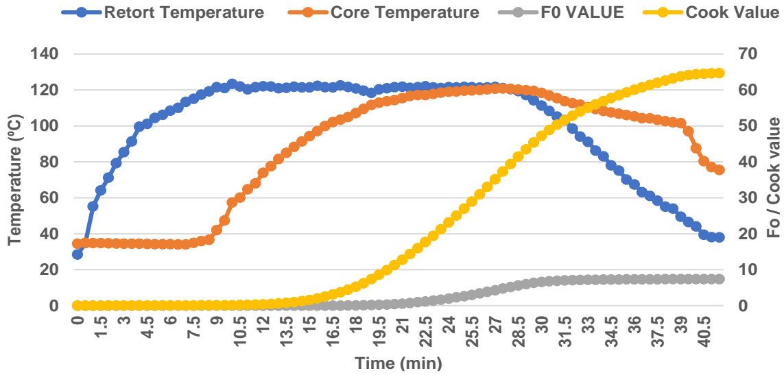
Fig. 1. Heat penetration rate, F_0 value and cook value of Pangasius fillet chunks in masala processed at F_0 7.37 min.
