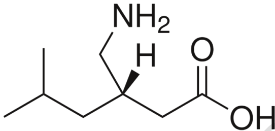
Figure 2: The chemical structure of Pregabalin [70].
