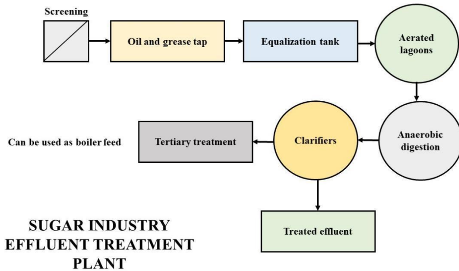
Figure 1: A Typical Effluent Treatment Plant
