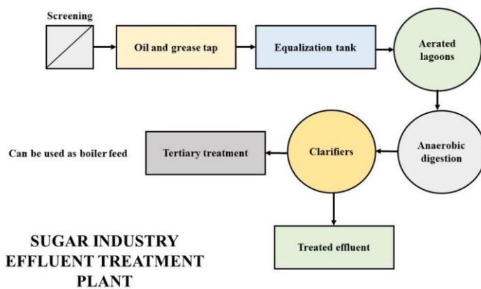
Figure 1: A Typical Effluent Treatment Plant
