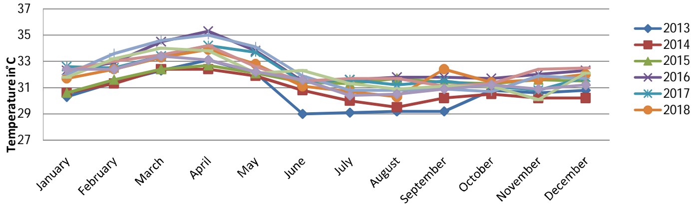
Figure 1 The graph depicting the month-by-month average maximum temperature from 2013-2018
