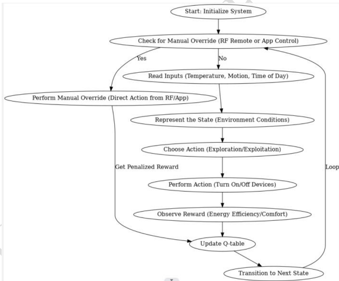
Figure 1. Reinforcement learning
