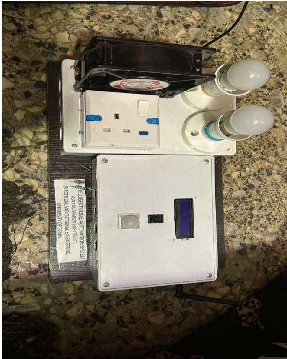
Figure 8. Automated Smart System (When Device is off)
