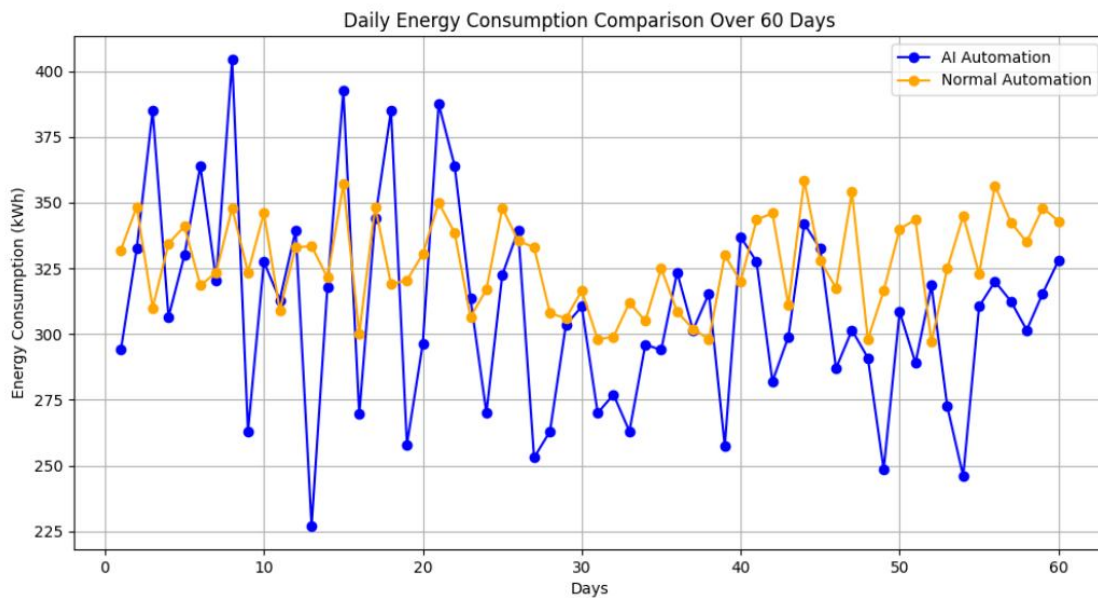
Figure 2. Daily Energy Consumption for 60 days
