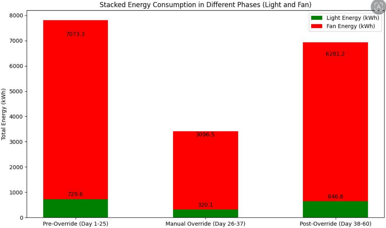
Figure 5. Energy Consumption in Phases (Light and Fan)
