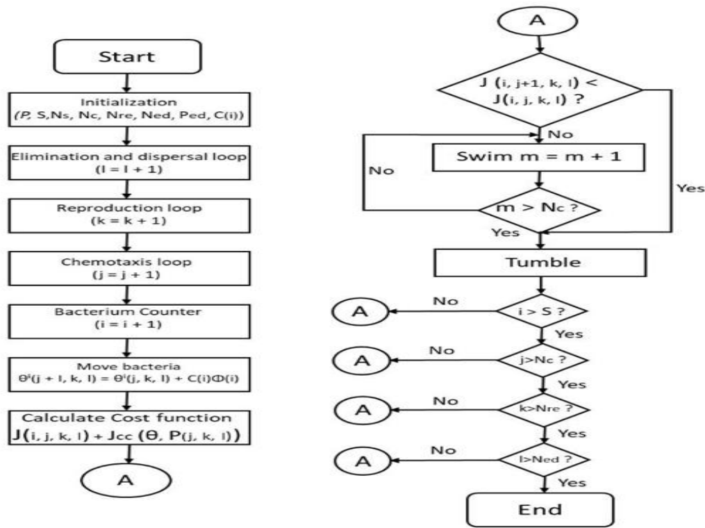
Figure 2: Flow chart of Bacterial Foraging Optimization Algorithm
