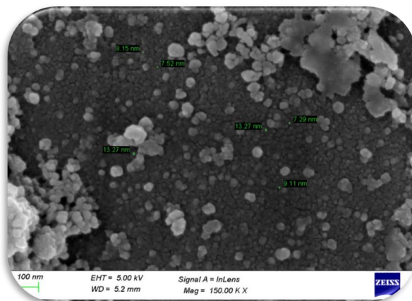
Fig. 4. Field Emission Scanning Electron Microscopy photograph showing a relatively spherical shape of mushroom nanoparticles in the range from 7.29nm to 13.27nm.
