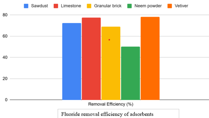
Fig – 1 Comparison of Fluoride Removal Efficiency Using Sawdust, Limestone, Granular brick powder, Neem leaf Powder, and Vetiver
