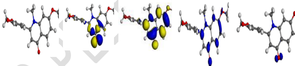
Figure 5: optimized structures, HOMO and LUMO orbitals, funki funtions of the selected compounds
