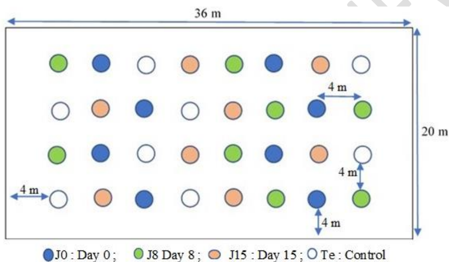
Figure 1 : Experimental set-up to study the effect of the order of appearance of L. siceraria berries
