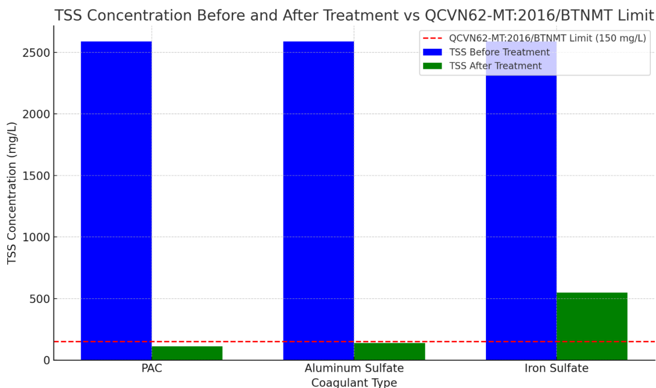
Fig 1: The TSS concentration of livestock wastewater samples before and after chemical treatment was evaluated and compared with QCVN 62-MT:2016/BTNMT
