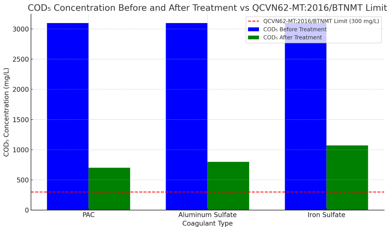
Fig 3: The COD 5 concentration of livestock wastewater samples before and after chemical treatment was evaluated and compared with QCVN 62-MT:2016/BTNMT
