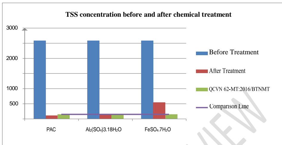
Fig 1: The TSS concentration of livestock wastewater samples before and after chemical treatment was evaluated and compared with QCVN 62-MT:2016/BTNMT
