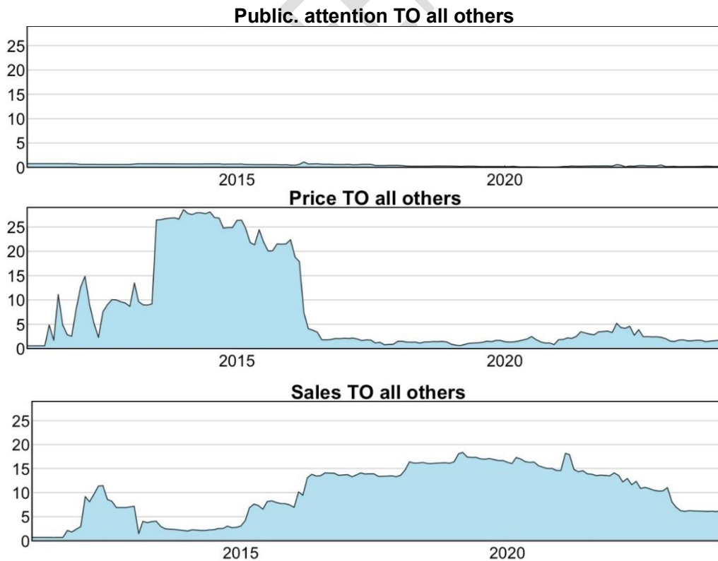
Fig. 5 Spillover effects of Public attention, House prices and Sales
