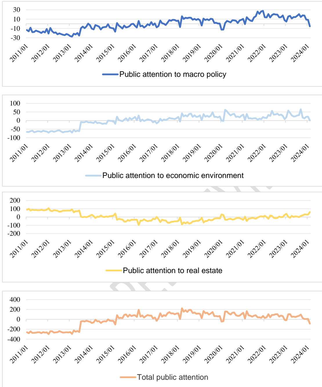
Fig. 2 Time series plots of the PCA for each type of data
