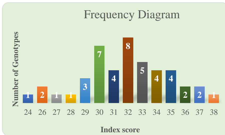
Fig. 4.3 Frequency Diagram of Index Score for 45 Greengram genotypes
