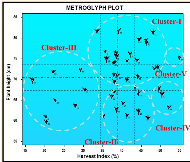
Fig. 4.2 Scatter diagram of Metroglyph Analysis
