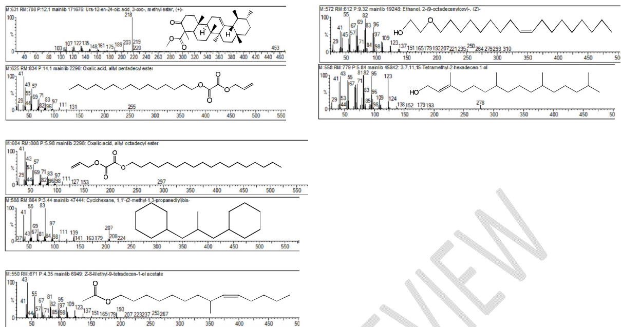
Fig. 4. Mass spectra of identified compounds from n-hexane fraction of T. catappa leaf extract
