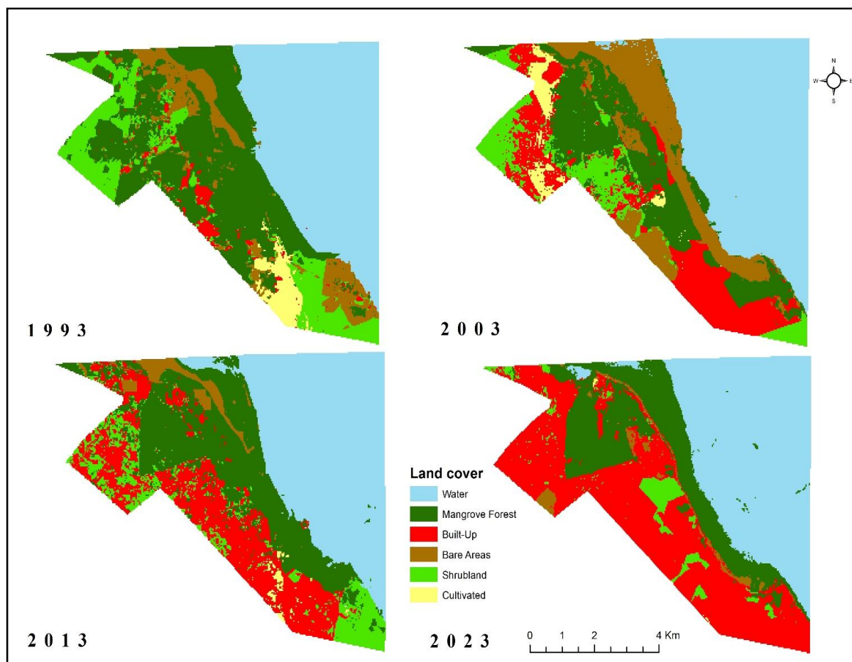
Figure 3: LULC for the years 1993, 2003, 2013 and 2023
