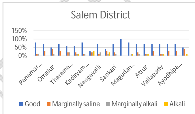
Fig. 4. Overall Percentage distribution of groundwater quality in Salem district
