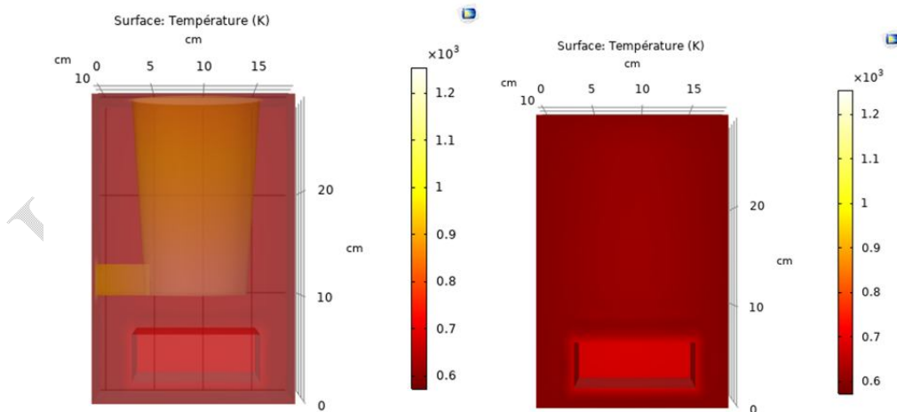
Figure 9: Heat propagation along the Z-X surface
