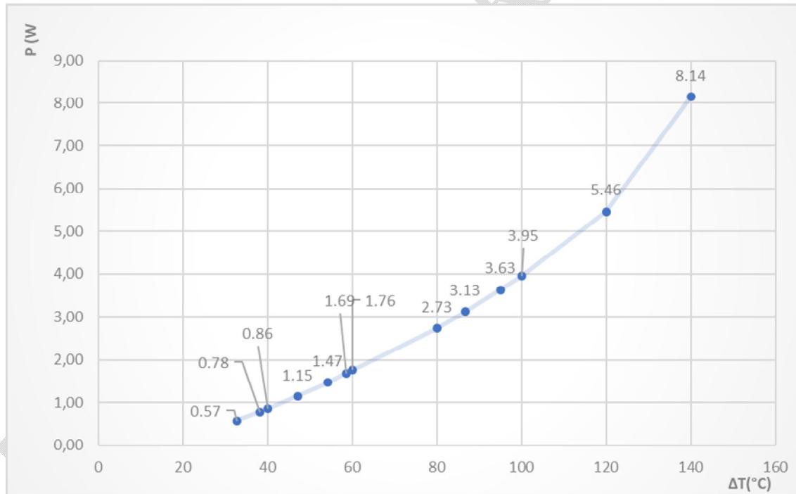
Figure 10: Practical power generated as a function of temperature difference
