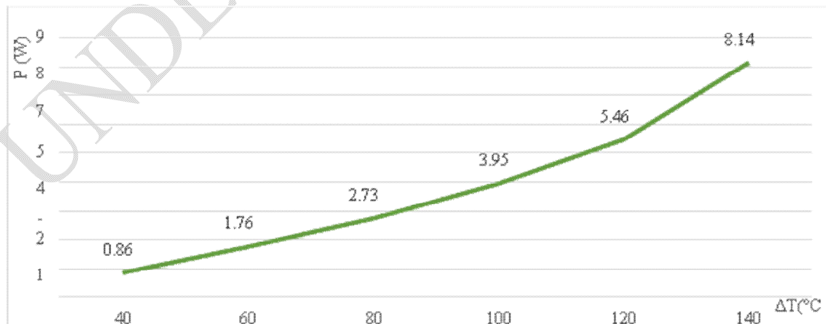
Figure 3: Representative curve of power generated as a function of temperature difference
