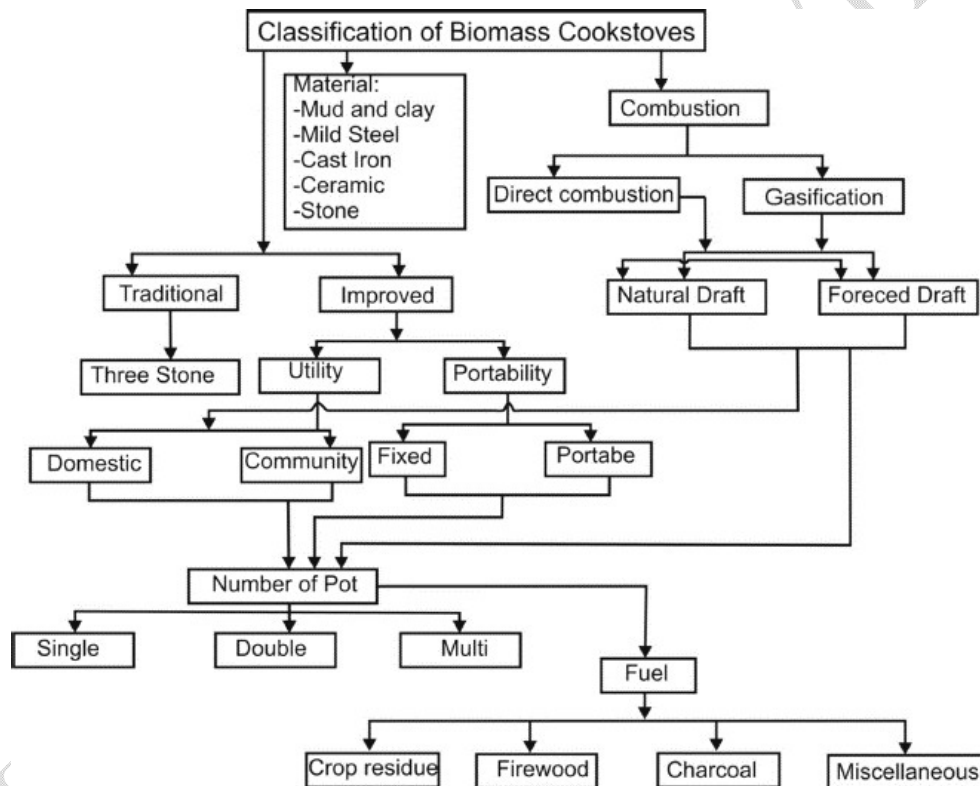
Figure 1: Classification of biomass cookstoves [16]
