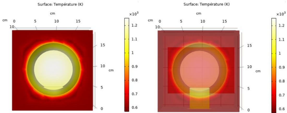
Figure 7: Heat propagation along the X-Y surface
