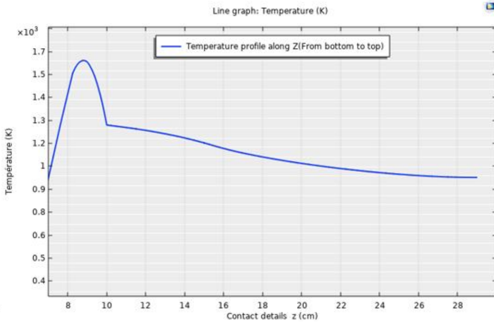
Figure 6: a) Temperature profile at the left wall of the furnace and b) Temperature profile inside the combustion chamber.
