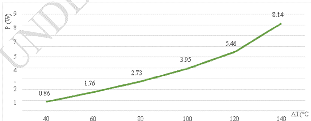
Figure 3: Representative curve of power generated as a function of temperature difference. The input parameters required for sizing the entire electrical system are shown in Table 4.
