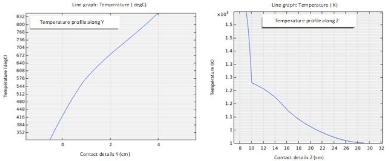
Figure 6: a) Temperature profile at the left wall of the furnace and b) Temperature profile inside the combustion chamber.
