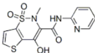
Scheme 1: Chemical structure of tenoxicam
