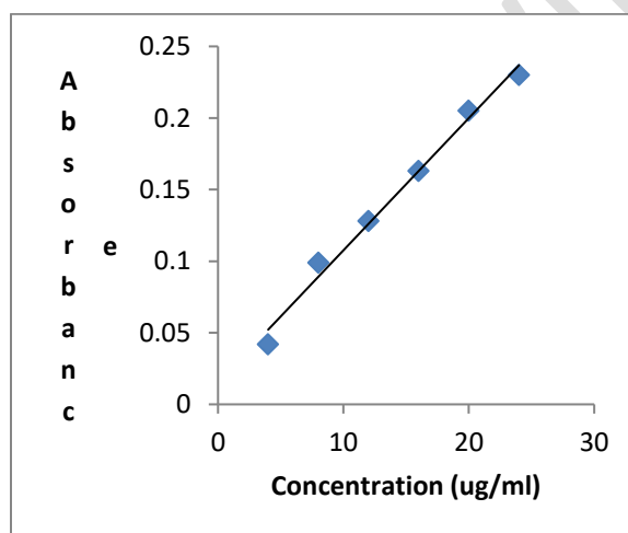
Figure 1. Calibration curve of tenoxicam
