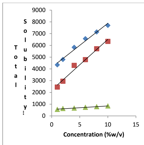
Figure 2: Plot of total solubility of tenoxicam versus hydrotrope concentration
