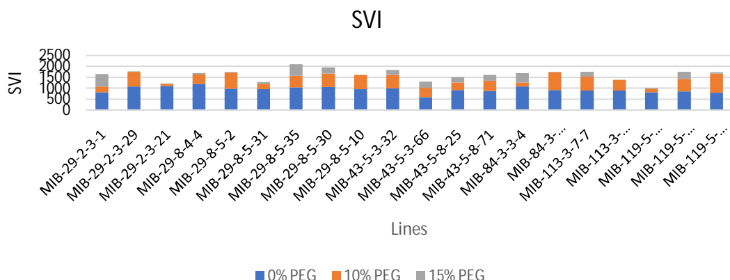
Figure 5. Effect of PEG on seedling vigour index (SVI) in different backcross inbred rice lines
