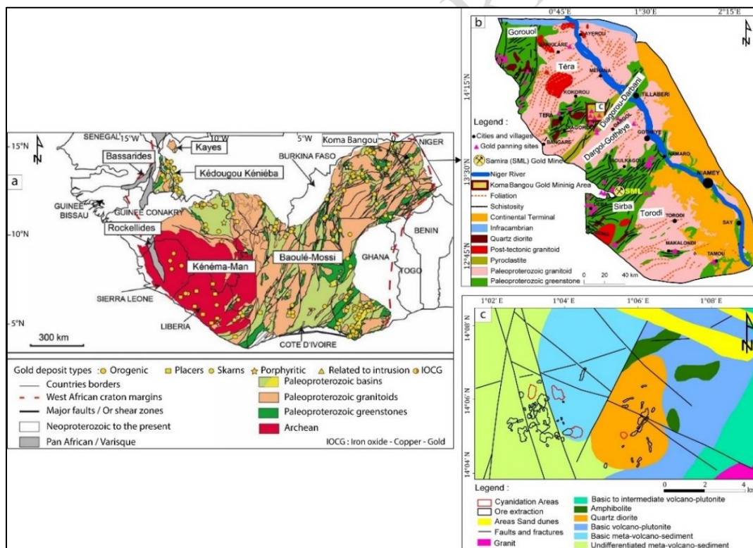
Fig. 1. a) Geological map of the Léo-Man ridge [31] and location of gold deposits [32]; b) Geological map of Liptako Niger [33]; c) Geological features of Koma Bangou [27].
