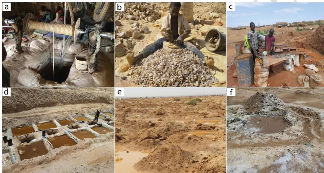
Fig. 2. Stages of artisanal gold mining at Koma Bangou. a) Ore extraction shaft fitted with winch; b) Manual crushing of ore; c) Gravity concentration of gold in sluice; d) Cyanide leach tanks for gold-bearing ore; e) Spreading of cyanidation waste; f) Acidification waste dump.
