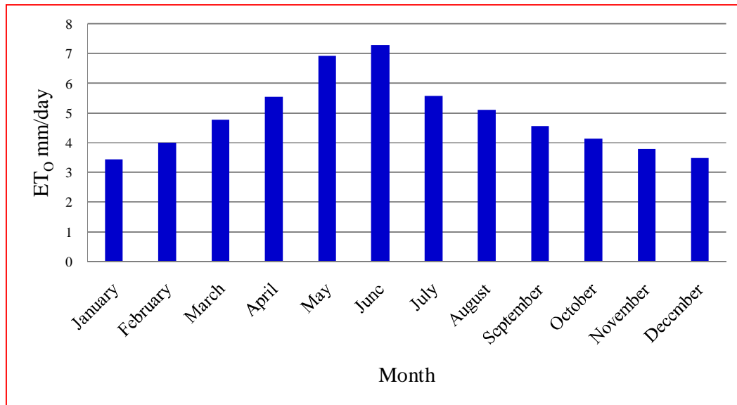
Fig. 1. Monthly ET 0 values of Krishna Central Delta
