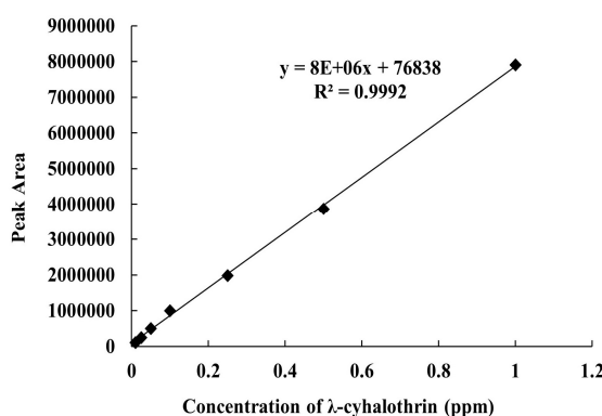
Fig. 1. Standard curve of \lambda -cyhalothrin on GC-MS/MS
