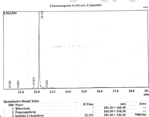
Fig. 2. Chromatogram of \lambda -cyhalothrin on GC-MS/MS
