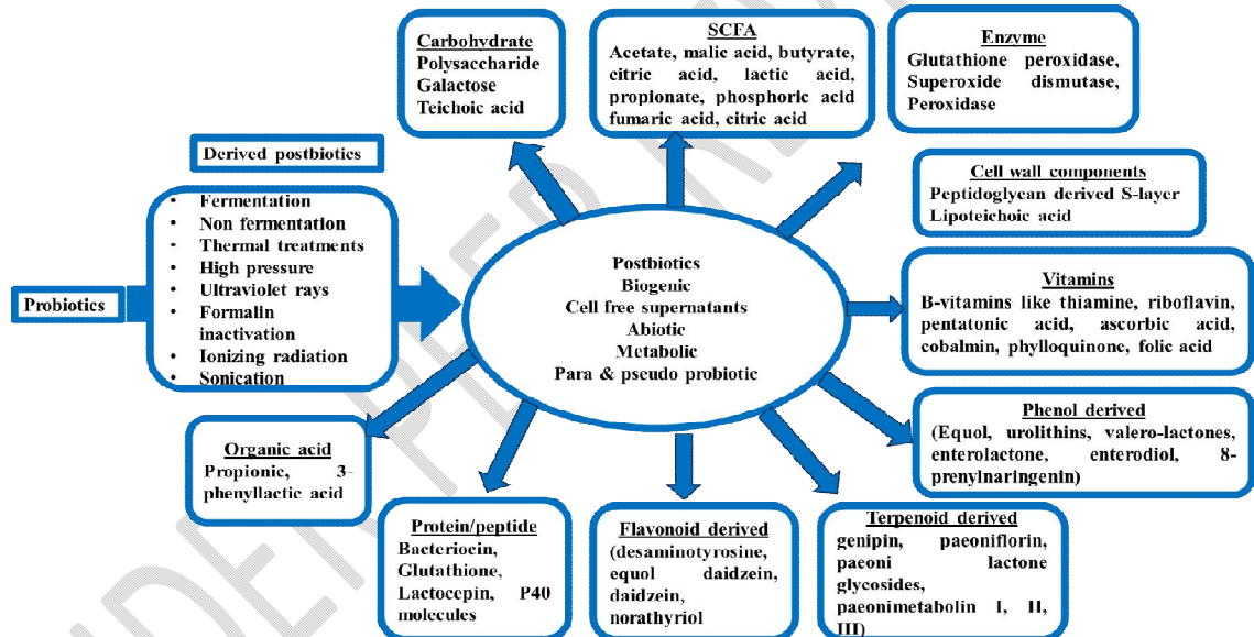
Fig 3. Main postbiotics generated by microbiota in colon and cecum
