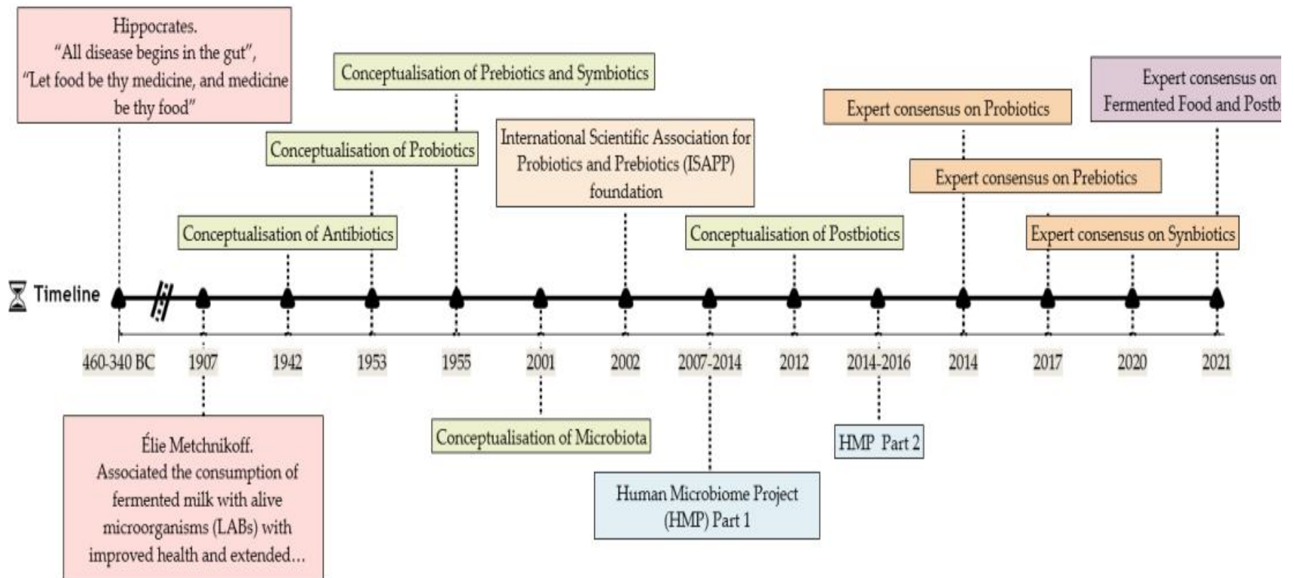
Fig 2. Timeline illustrating the main historical milestones in microbiology (Cabello-Olmo et al., 2021)
