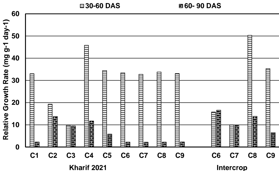
Fig.4 Effect of cropping system on relative growth rate ( \text{mg g}^{-1} \text{ day}^{-1} ) under natural farming during kharif 2021
