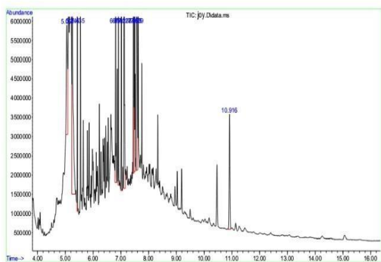
Figure 9: Extract GC-MS Scan
