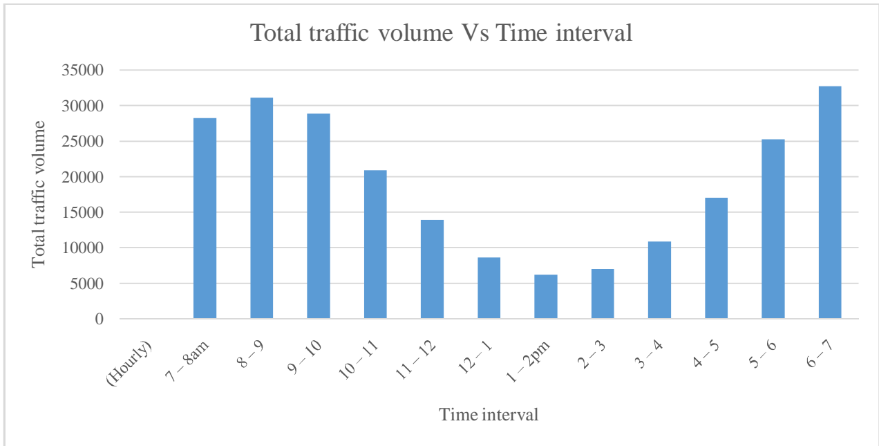
Fig.2: Graphical representation of total traffic volume against hourly time interval at Rumuokwuta junction
