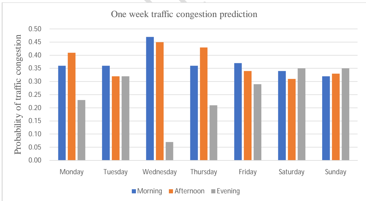
Fig.5: Naïve Bayes' traffic congestion prediction for daily session
