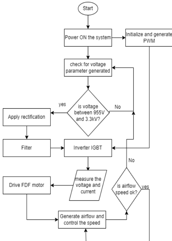
Fig.5: Flowchart of the proposed VFD control
