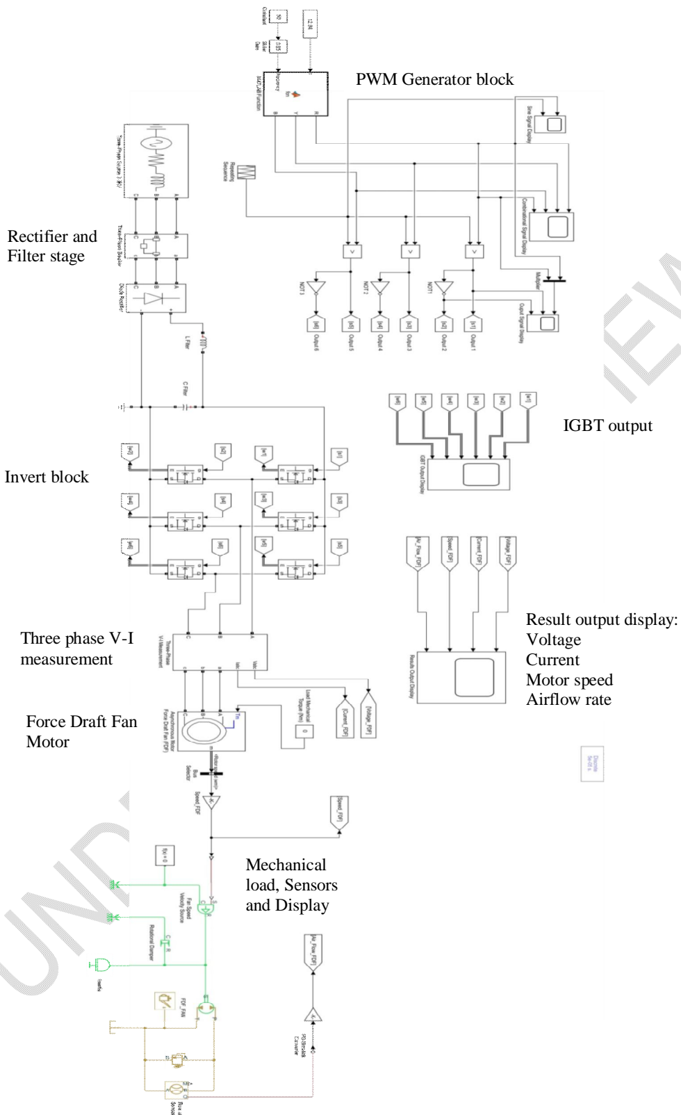
Fig. 4: Simulated blocks of the VFD control system
