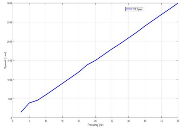
Fig.6: Correlation between Frequency (input) and Speed of the VFD FDF
