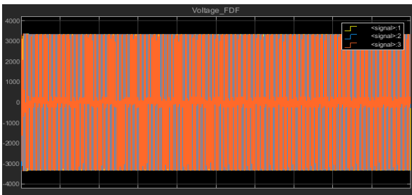
Fig. 9: VFD Simulation Voltage Output Result
